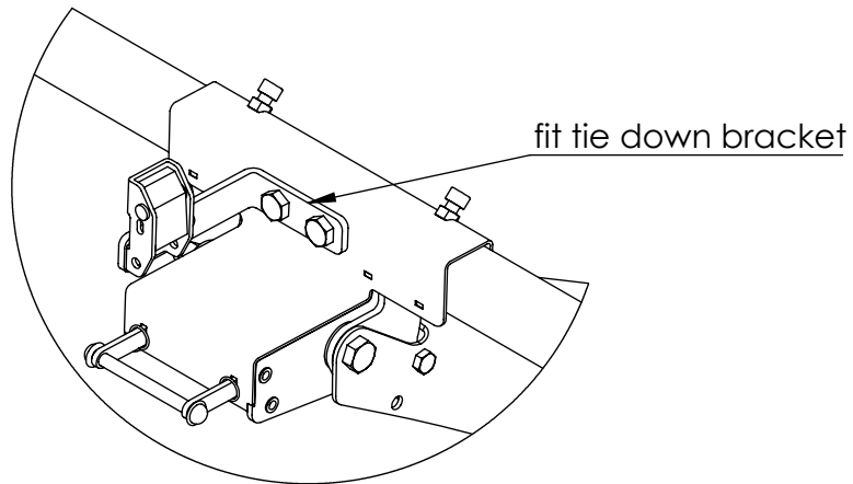
Tie down bracket with strap x 1
